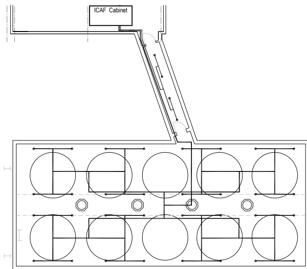
Figure 1: Detail of the CAF Nozzles balanced layout.
